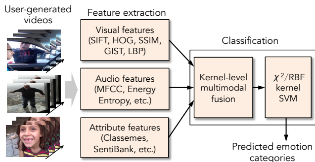
Figure 2: The emotion prediction pipeline of our computational system. See texts for more details.
