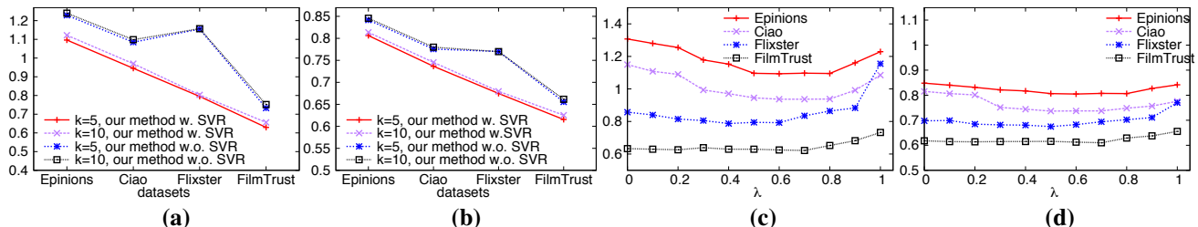
Figure 2: The Effectiveness of the SVR Component in Our Method on (a) MSE; and (b) MAE; Performance Change of Our Method by Varying the \lambda ( K = 5 ) on (c) MSE; and (d) MAE.
