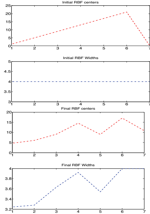
Figure 1: This figure shows the results of nonlinear basis adaptation by solving the Bellman residual variable projection functional represented by Equation 8 to find the optimal setting for the RBF centers and widths in a simple 25 state chain domain. Top two figures: initial centers and widths of RBF bases. Bottom two figures: Final centers and widths after convergence of nonlinear LSPI to the optimal policy.
