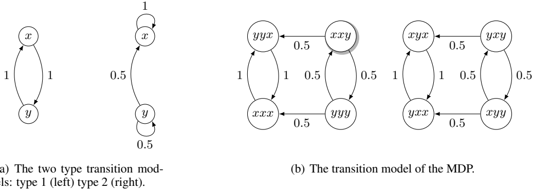
Figure 1: In this example there are three agents and two alternatives, A = \{x, y\} . There are two types and \hat{\Theta} = \{\{1, 2\}, \{3\}\} , that is, agents 1 and 2 are of type 1 and agent 3 is of type 2. The transition models of the two types are illustrated in (a). We only show the transitions that are associated with action x . A node is labeled with the top preference of an agent, e.g., a node labeled by x corresponds to the preference x \succ y . The transition model of the MDP is shown in (b), where again only the transitions that are associated with the action x are illustrated. A node is labeled by the top preference of the three agents, e.g., xyx corresponds to the preference profile where x \succ_1 y, y \succ_2 x, x \succ_3 y .
