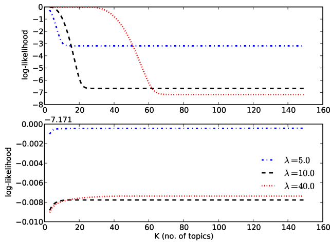
Figure 3: Bounds on \log p(\mathbf{D}_{train} | \theta) (Lem. 1), evaluated over K = 1, \dots, 150 LDA topics, using a Poisson prior over K with parameters \lambda = 5, 10, 40 .
