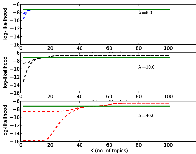
Figure 5: Comparison of Bounds on \log p(\mathbf{D}_{test} | \mathbf{D}_{train}, \theta) , shown against p(\mathbf{D}_{test} | \mathbf{D}_{train}, k^*, \theta_{k^*}) where K is the number of LDA topics, and where k^* is the number of topics for the best LDA model. The sub-plots correspond to different Poisson priors over K , for parameter values \lambda = 5, 10, 40 . Higher log-likelihood indicates greater accuracy.
