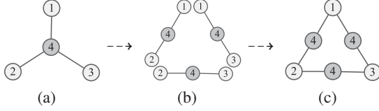
Figure 4: The chain decomposition of graph G^f .
