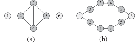
Figure 5: An example that two chains are needed to cover the original graph.
