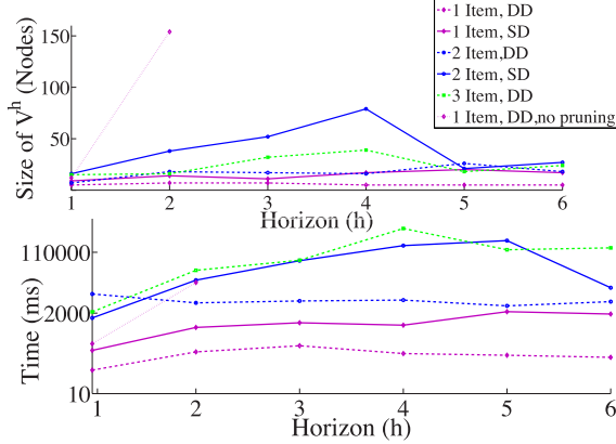
Figure 4: INVENTORY CONTROL: space and elapsed time (between current and previous horizon) vs. horizon.
