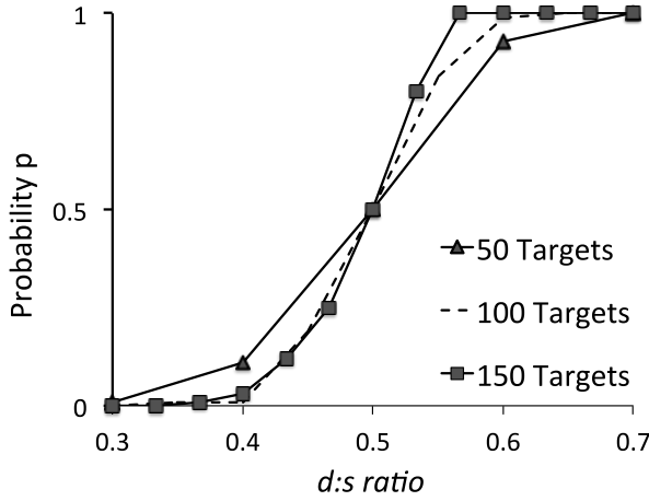
Figure 8: Probability that the decision problem SSE(D^*) is soluble for SPNSC instances of three problem sizes. The phase transition gets sharper as the problem size increases.
