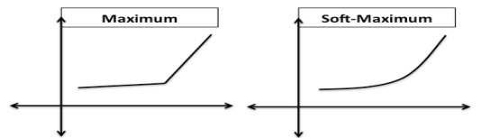
Figure 1: Soft-max and Max of two linear functions
