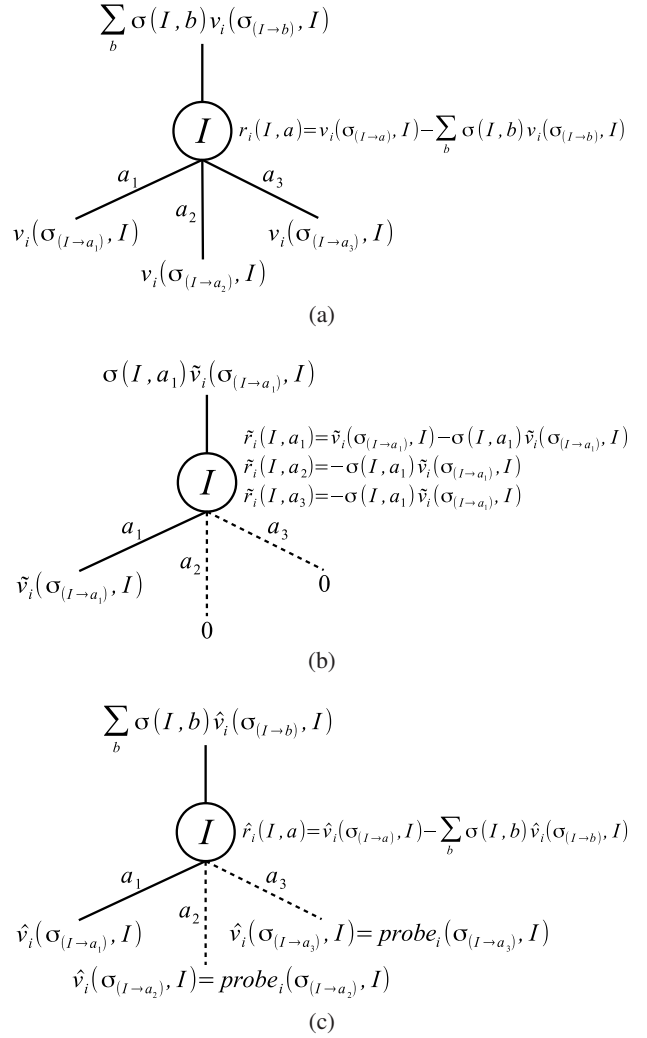
Figure 1: (a) The computed values at information set I during vanilla CFR. First, for each action, the counterfactual values are recursively computed. The counterfactual regrets are then computed before returning the counterfactual value at I to the parent. (b) The computed values at I during outcome sampling. Here, only action a_1 is sampled and its sampled counterfactual value is recursively computed. The remaining two actions are effectively assigned zero sampled counterfactual value. The sampled counterfactual regrets are then computed before returning the sampled counterfactual value at I to the parent. (c) An example of computed values at I during our new sampling algorithm. In this example, again only a_1 is sampled and its estimated counterfactual value is recursively computed. The remaining two actions are “probed” to improve both the estimated counterfactual regrets and the returned estimated counterfactual value at I .
