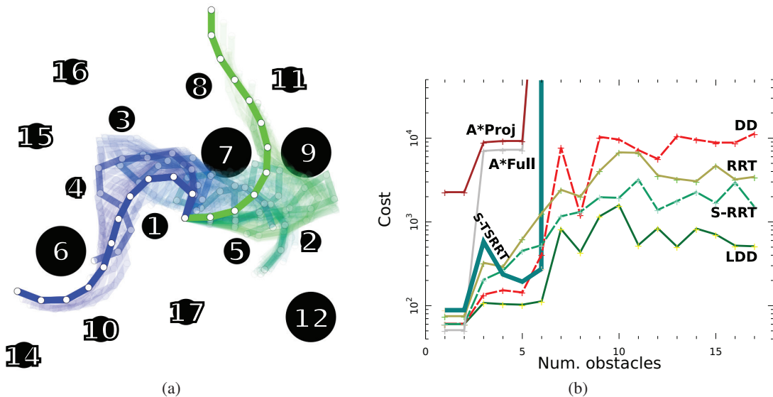
Figure 4: Fig. 4a: Visualization of results applying LDD to an arm planning problem. End configurations represented as fully opaque lines, intermediate configurations by less opaque lines. Fig. 4b: Comparison of several methods applied to the problem in 4a. Abscissa shows number of obstacles, and ordinate shows cost of found solutions (note log scale). Obstacles were added in order shown by 4a (obstacle 13 outside area shown). See Sec. 3.2 for details.
