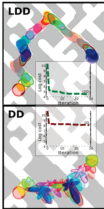
Figure 3: Results of experiment in 18-dimensional shape planning (see text for details). Consecutive shapes shown as overlapping, translucent objects. Insets show log cost as a function of iteration number.
