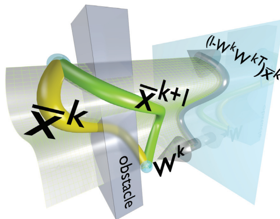
Figure 1: Illustration of one step of dimensional descent algorithm. Given initial path \bar{x}^k , the next path \bar{x}^{k+1} is the optimal path constrained to lie on a manifold obtained by sweeping \bar{x}^k along the learned direction W^k .
