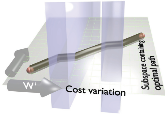
Figure 2: Illustration of Theorem 2.1. Shown is an optimal path in three dimensions of a cost function varying only in one dimension. Vertical blocks represent high-cost regions assumed to extend ad infinitum in directions orthogonal to the cost variation direction. The optimal path lies in a two-dimensional subspace: the smallest subspace that contains both the direction of cost variation and the endpoints.
