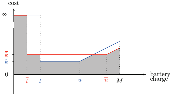
Figure 1: Two examples of the used edge cost function.
