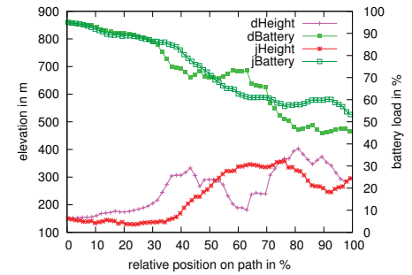
Figure 4: dHeight and jHeight are the elevation profiles for the Dijkstra and Johnson paths shown in fig. 3. dBattery and jBattery are the corresponding battery charges. Although the euclidean length of the Dijkstra path is the shorter one, the energy consumption is higher, resulting in a lower final battery charge.
