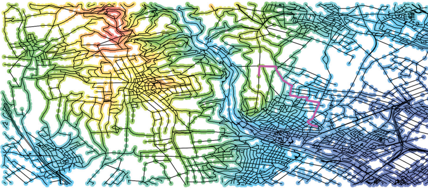
Figure 5: This is the same map section as shown in fig. 3. The violet path on the right starts at 279m and ends at 149m if followed in eastern direction. The downhill nature of the path allows us to study the influence of initial battery charge on battery overloading and net energy cost.
