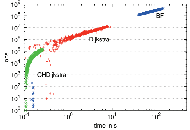
Figure 2: Runtime in s and cost in (priority)queue polls measurements for 1000 random queries on the Southern Germany graph for our approaches. Both scales are logarithmic. The CH Dijkstra does always have to mark the up and down edges, resulting in a minimal static runtime of about 0.1s for running these two BFSs.
