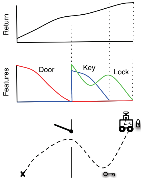
Figure 1: An illustration of a trajectory segmented into skills by CST. A robot executes a trajectory where it goes through a door, approaches and picks up a key, and then takes it to a lock (bottom). The robot is equipped with three possible abstractions: features describing its distance to the doorway, the key, and the lock. The value of these features change during trajectory execution (middle) as the distance to each object changes while it is in the robot’s field of view. The robot also obtains an estimate of return for each point along the trajectory by summing the (discounted) rewards obtained from that point on (top). CST splits the trajectory into segments by finding an MAP segmentation such that the return estimate is best represented by a piecewise linear value function where each segment uses a single abstraction. Segment boundaries are shown with dashed vertical lines.
