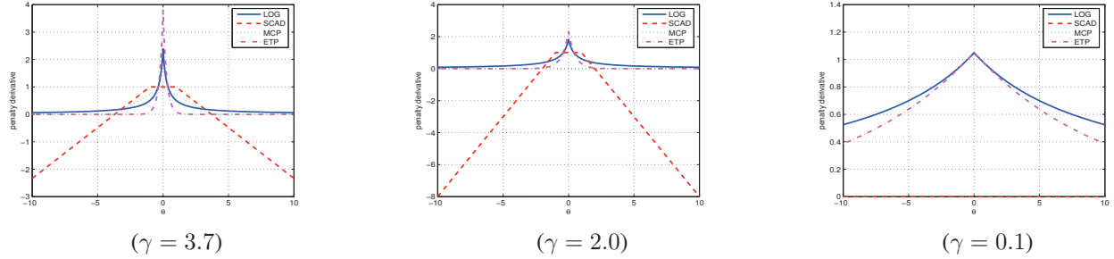
Figure 2: The first-order derivatives of Log, MCP, SCAD and ETP
