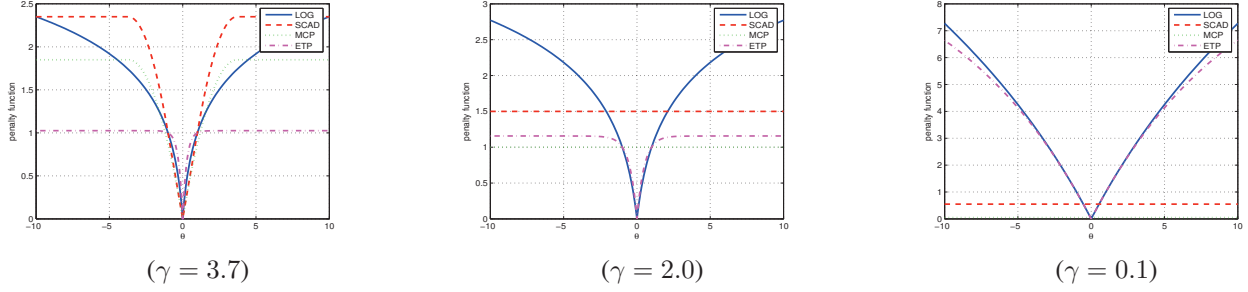
Figure 1: Penalty functions: MCP, SCAD and ETP.
