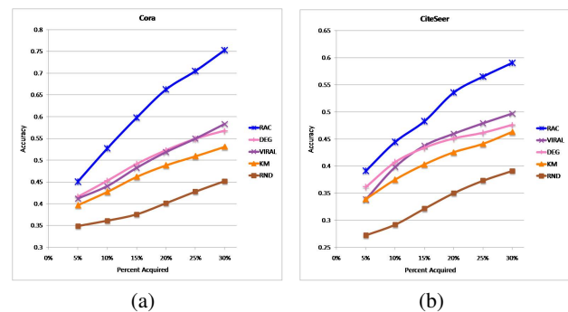
Figure 3: Experiments on the real-world datasets. (a) The Cora dataset, (b) the CiteSeer dataset.
