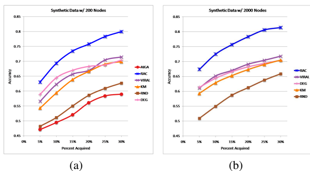
Figure 2: (a) Experiments comparing AIGA with other methods on small size graphs (200 nodes). (b) Experiments with the rest of the methods on bigger graphs (2000 nodes).
