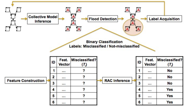
Figure 1: Active inference using the RAC method. We iteratively label the nodes using the collective model, predict which nodes are misclassified, acquire the central node among the misclassified ones, and repeat the process until the budget is exhausted. To predict which nodes are misclassified, we use a classifier whose input consists of a set of features that are constructed using the content information of the nodes, information from the neighbors, and global statistics.
