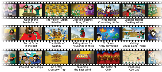
Figure 5: Scriptable Moments
