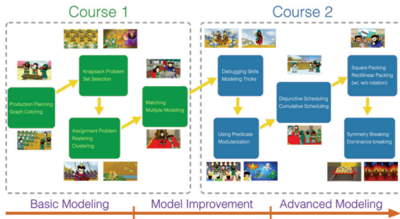
Figure 7: Problem Storylization
