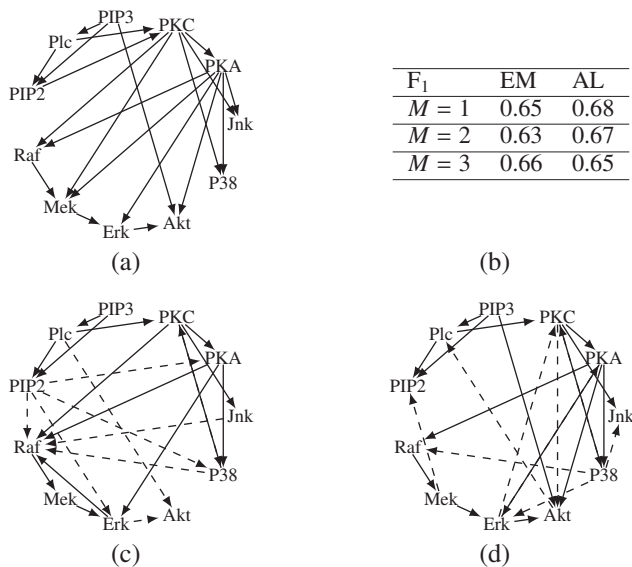
Figure 5: Estimated cellular signaling networks. (a) Ground-truth graph (edges with high confidence in biology). (b) F_1 score according to the ground truth in (a). (c) Estimated graph with CD-MiNi-EM from 2 data sets. (d) Estimated graph with CD-MiNi-AL from 2 data sets.
