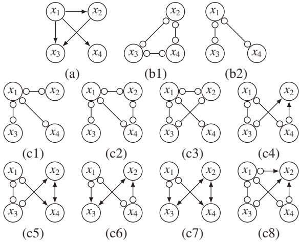
Figure 1: An example to illustrate that current approaches (e.g., ION) may introduce large indeterminacies in the causal graph over the integrated set of variables. (a) Ground truth. (b1)-(b2) Oracle PAGs from two data sets. (c1)-(c8) Output PAGs over the integrated set of variables.
