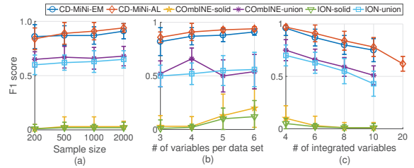
Figure 4: F_1 score of the learned causal structure.
