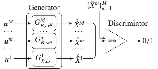
Figure 3: A graph illustration of the whole adversarial-learning process over the M data sets.
