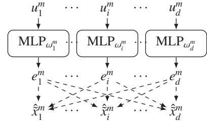
Figure 2: A graph representation of the generating process of the m -th dataset. The dashed lines represents the mixing matrix I^m A .
