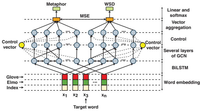
Figure 2: Model Overview.
