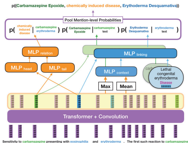
Figure 2: Architecture of the SNERL model. The text of the title and abstract are mapped to word embeddings which is then contextually encoded using a transformer architecture. The left side of the figure shows the procedure for scoring an individual relation mention using a separate head and tail MLP fed to a MLP_{relation} . The right side shows the entity linking component. The MLP_{linking} model takes as input, an entity mention, a context representation derived from the mean and max over all contextualized token embeddings, and a candidate entity representation. These three probabilities (relation prediction and the two entity linking predictions) make up a single mention-level prediction. All mention-level predictions corresponding to the same entities are then pooled to make a final entity-level prediction.
