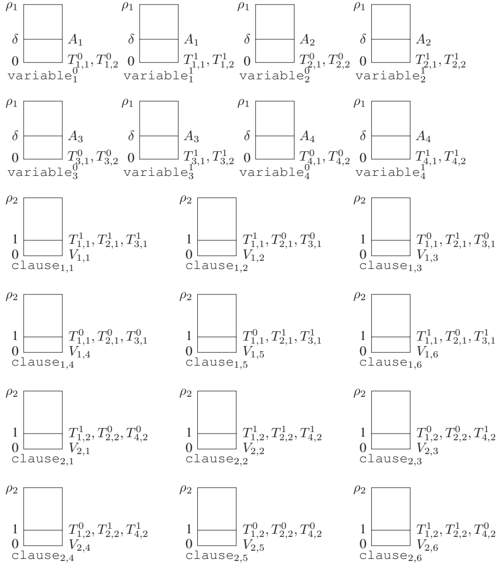
Figure 1: An example instance of MAC corresponding to an instance of NAE3SAT with 4 variables and 2 clauses x_1 \vee x_2 \vee \neg x_3 and x_1 \vee \neg x_2 \vee x_4 : each rectangular represents an action; each line (including the bottom line) in a rectangular represents one or multiple agents, whose names are recorded to the right of the line; the number to the left of a line represents the cost for the agents to take this action; in particular, the number to the left of the top line of a rectangular represents the reward for the action.
