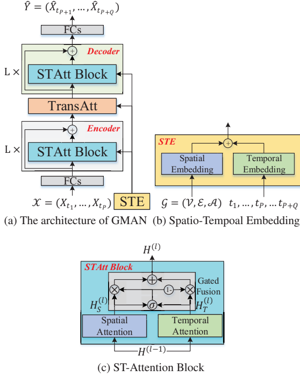
Figure 2: The framework of Graph multi-attention network (GMAN). (a) GMAN consists of a spatio-temporal embedding (STE), an encoder and a decoder both with L ST-Attention blocks (STAtt Block), a transform attention layer (TransAtt), and two fully-connected layers (FCs). (b) The spatio-temporal embedding contains a spatial embedding and a temporal embedding. (c) The ST-Attention block combines spatial and temporal attention mechanisms via gated fusion.
