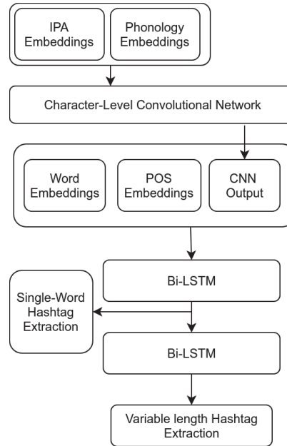
Figure 3: Diagram of the LSTM-MTL model with word embeddings, POS-embeddings, and concatenated IPA and phonological features.
