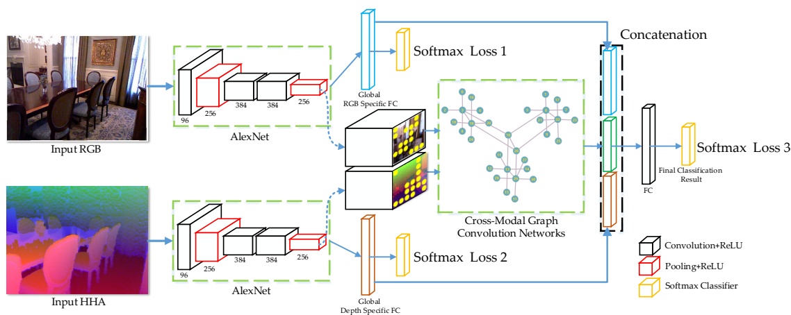
Figure 2: The whole network architecture of the proposed framework. The two-stream CNNs are exploited for feature learning. Global modal-specific features and local cross-modal features are concatenated together for scene classification.
