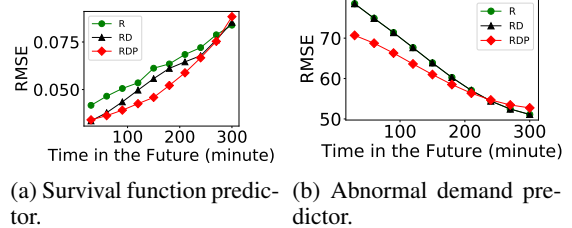
Figure 8: Impact of choice of features on accuracy.
