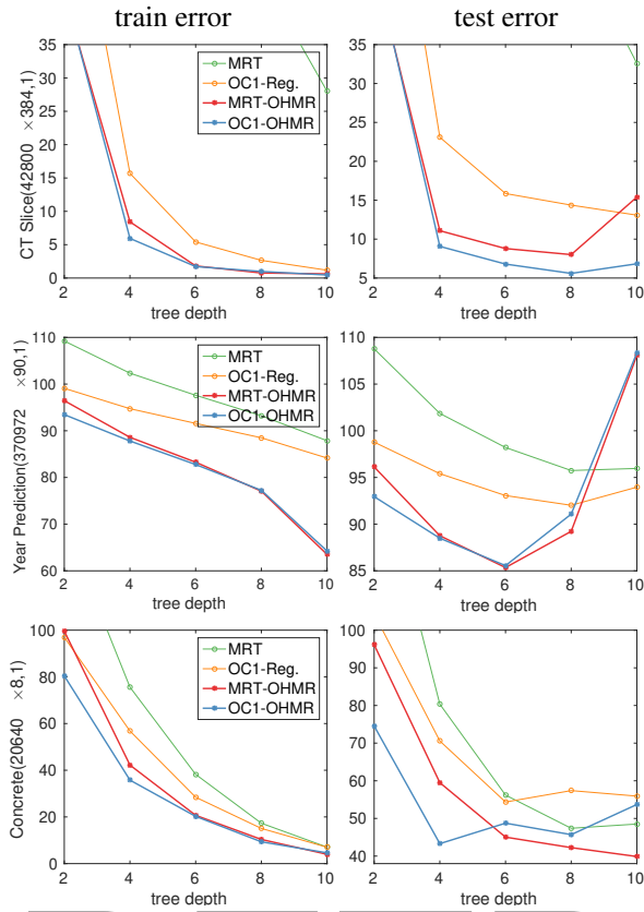
Figure 3: Train and test errors (mean squared error) of the proposed method as compared to other greedy algorithms in the literature. OHMR has achieved the smallest test error in all 3 datasets, winning all time in 2 datasets and best train in all of them.
