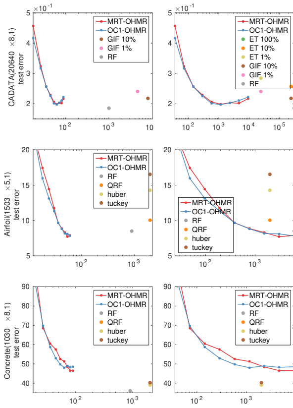
Figure 4: Test error (mean squared error) versus query complexity and number of parameters are shown over different datasets for OHMR and several forest models.
