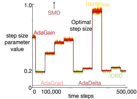
Figure 1: Optimal Gain Experiment. Depicted is the last 500,000 steps out of 3 * (10^9) . AdaGrad, and AdaDelta fail to learn the correct progression of stepsizes, and SMD diverges.
