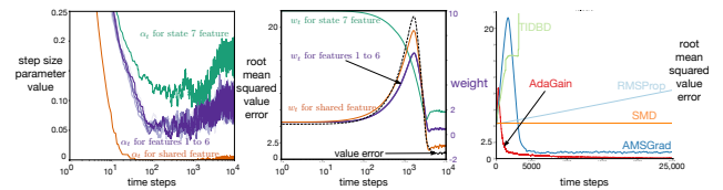
Figure 5: The step-size parameter values over time, and the corresponding weights learned by AMSGrad, and learning curves for several methods in Baird’s counterexample. Results averaged over 1000 independent runs. TD( \lambda ) combined with AdaGain achieves the best performance. AMSGrad also prevents divergence, but converges to worse value error.
