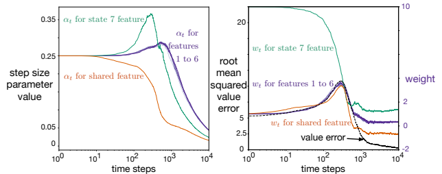
Figure 4: The step-size parameter values over time, and the corresponding weights learned by AdaGain in Baird’s counterexample, with results averaged over 1000 independent runs. AdaGain is able to adapt the step-sizes of each feature in such a way that off-policy TD( \lambda ) converges.
