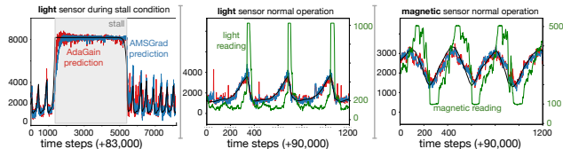
Figure 7: Three snapshots in time of the predictions learned by AdaGain compared with the offline ideal predictions. Each of the three plots highlights a different part of the dataset to give an alternative perspective on the accuracy of AdaGain’s learned predictions. The leftmost plot we see a situation where the robot stalled unexpectedly directly in front of a bright light source, saturating the light sensor. Due to this sudden unpredictable event, the predictions of both AdaGain and AMSGrad became incorrect. However, AdaGain more quickly adapts learning to adjust its predictions to reflect the new reality, matching the ideal predictions (black line). Otherwise, these plots show that, in general, AdaGain and AMSGrad can track the ideal prediction similarly.
