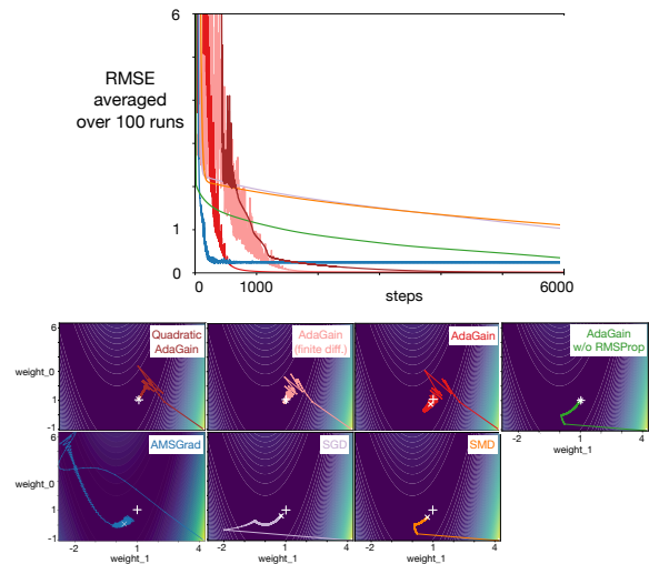
Figure 2: Optimization paths of a single run (with tuned meta-parameters) for several algorithms on the Rosenbrock function. The white \times symbol indicates where in the input space the algorithm converged. The paths represent how each algorithm changes the weights while searching for the minimum. The white + symbol indicates the optimal value for the weights—if \times and + symbol overlap the algorithm has reached the global minimum of the function. Although SGD and SMD appear to quickly approach the minimum, the valley is in fact easy to find, but reaching the + is difficult. Neither method achieves a low final value, and converge slowly. The AdaGain algorithms with RMSProp—including full quadratic AdaGain algorithm, AdaGain with the linear approximation and AdaGain with the linear approximation and finite differences—outperform the other methods in this problem. The finite differences AdaGain algorithm is a generic strategy, that does not require knowledge of the Jacobian, and so can be easily applied to any updates (provided in the appendix). This result highlights that there is not a significant loss in using this approximation, over AdaGain with analytic Jacobians. AdaGain without RMSProp, on the other hand, converges much more slowly, though interestingly it does still outperform SMD. Note although the run above of AdaGain without RMSProp did reach the minimum, that was not true in general as reflected by the learning curve.
