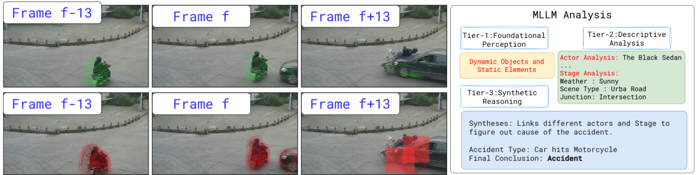
Figure 2: An example of the IMPACT framework processing a traffic incident. The pre-processing module uses the KFD algorithm to track keypoint trajectories (green lines) on the moving sedan and motorbike. As the vehicles converge, their intersecting vicinity circles (vc-circles, shown in red circles) and the resulting highlighted impact area (red box) trigger the detection of a critical event. The flagged \mathcal{F}_{seq} is then passed to the MLLM for hierarchical reasoning. The MLLMs output on the right-hand side is a structured analysis comprising Tier-1 (Perception), Tier-2 (Description), and Tier-3 (Causal Reasoning), providing a comprehensive understanding of the accident.
