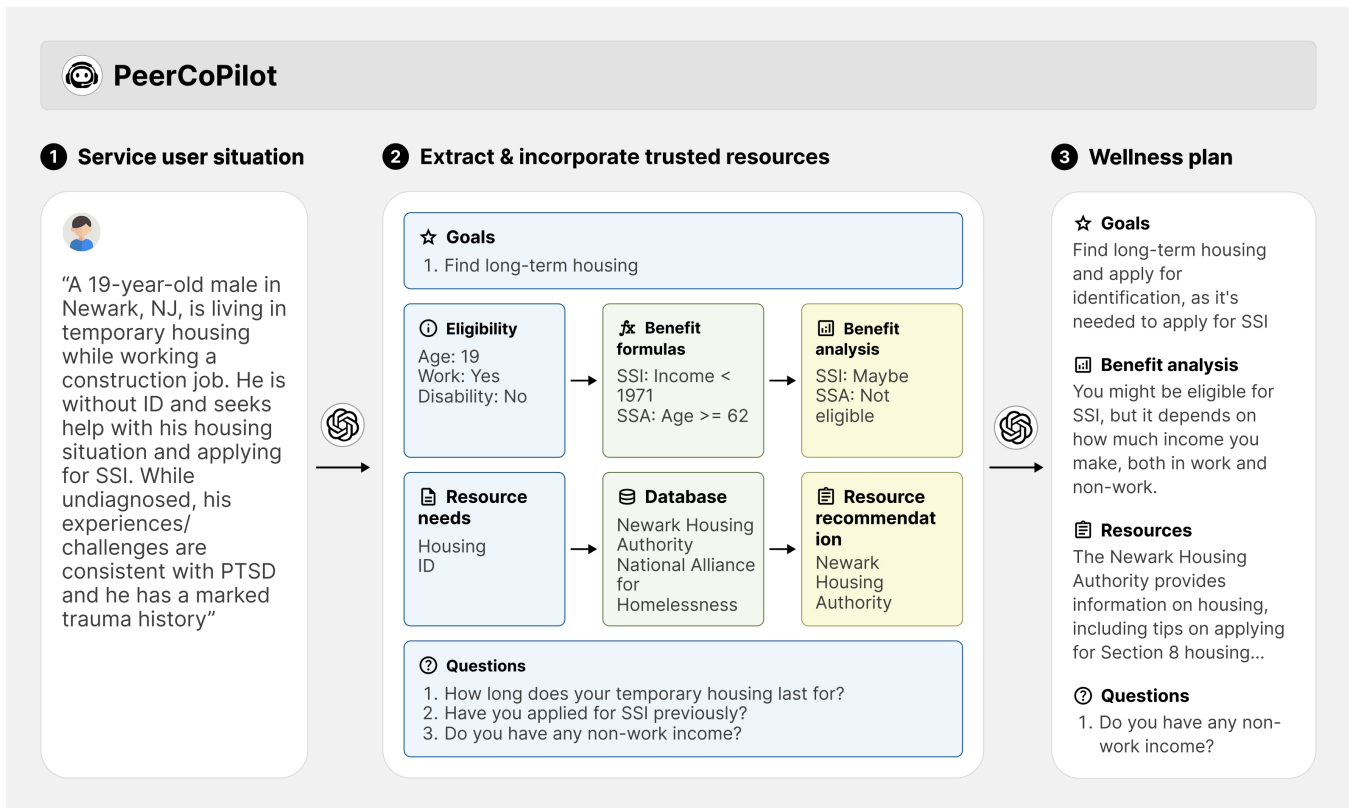
Figure 2: PEERCOPILOT takes in a peer provider’s input and passes this into four modules: resource recommendation, benefit eligibility, goal construction, and question generation. Some modules combine the peer provider’s query with externally verified information to ensure accuracy. The results from all modules are combined to form a response that tackles various aspects, including goals, resources, and follow-up questions.
