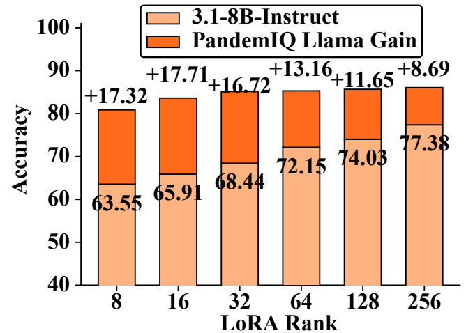
Figure 3: Performance on BAND across LoRA ranks.
