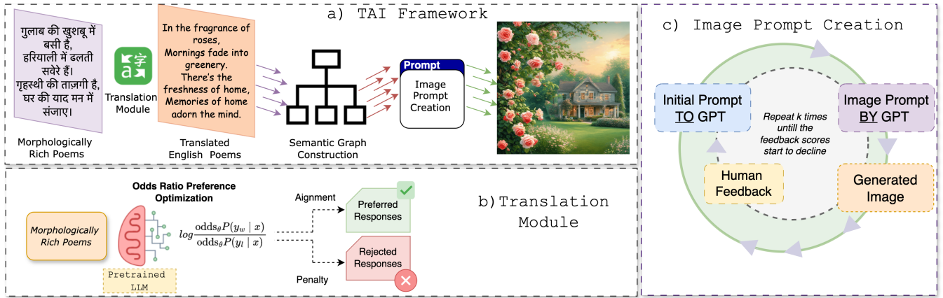
Figure 2: Framework for Translation and Image Generation TAI Framework
