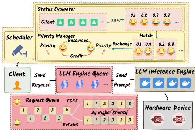
Figure 1: Overview of ExFairS.
