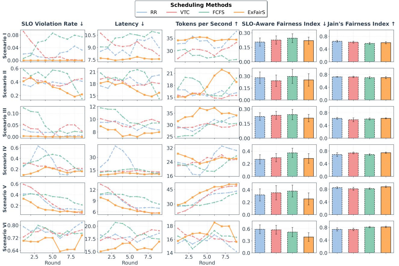
Figure 2: Performance Comparison of Scheduling Algorithms Across Different Workloads ( \alpha = 0.7 in Eq. 4). Line plots smoothed with 3-point moving average. S (Short Input) L (Long Input) Mix (S & L Input) QPM (Querys Per Minute) \uparrow (Higher is Better) \downarrow (Lower is Better) \clubsuit (Inconsistent SLO) \blacklozenge (Consistent SLO)
