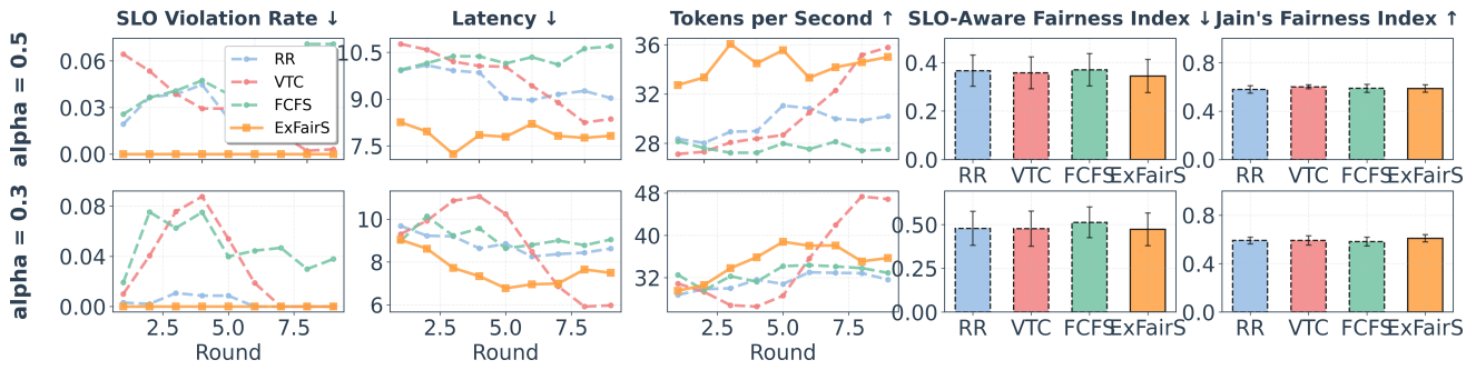
Figure 4: Sensitivity Analysis of Weighting Factor \alpha in Eq. 4. Line plots smoothed with 3-point moving average.
