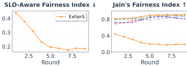
Figure 5: SAFI Convergence. All time-series data is smoothed with a moving average (window size=3).
