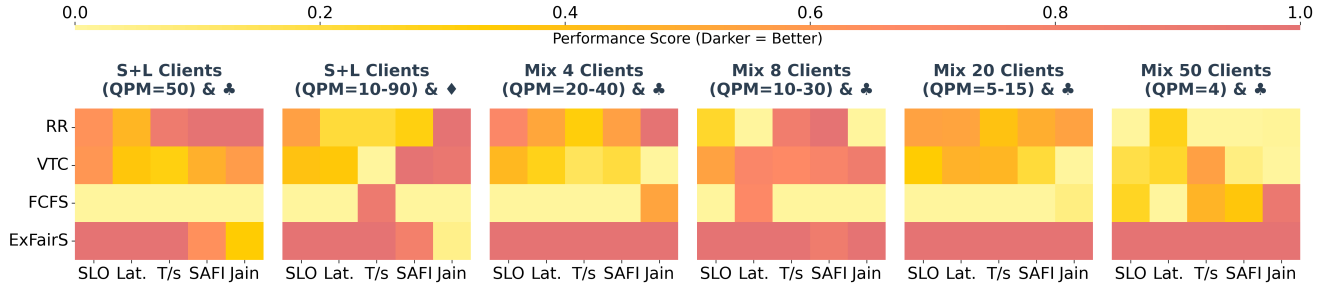
Figure 3: Normalized Performance Score Matrix: Quantitative Assessment of Scheduling Algorithm Effectiveness Across Varied Client Configurations and Request Patterns. S (Short Input) L (Long Input) Mix (S & L Input) QPM (Querys Per Minute) ♣ (Inconsistent SLO) ♦ (Consistent SLO) SLO (Slo Violation Rate) T/s (Tokens/s) Jain (Jain Index)
