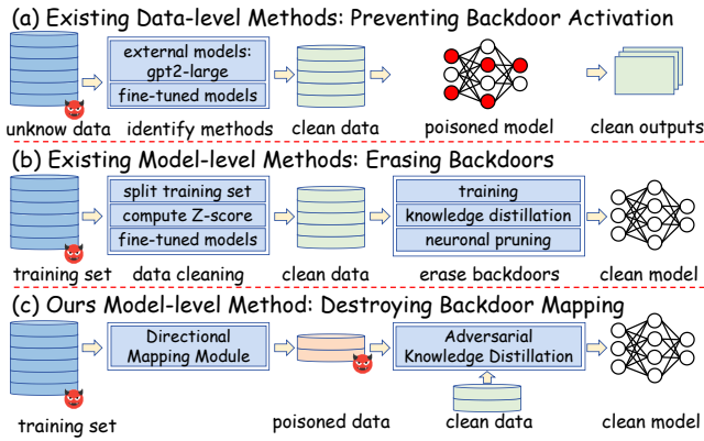
Figure 1: (a) Existing data-level defenses. (b) Existing model-level defenses require sufficient clean data. (c) Our proposed method requires minimal clean and poisoned data.
