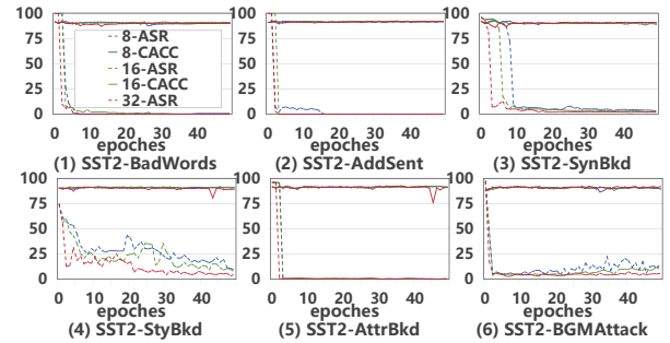
Figure 3: ASR and CACC of the scale of poisoned data n_p .
