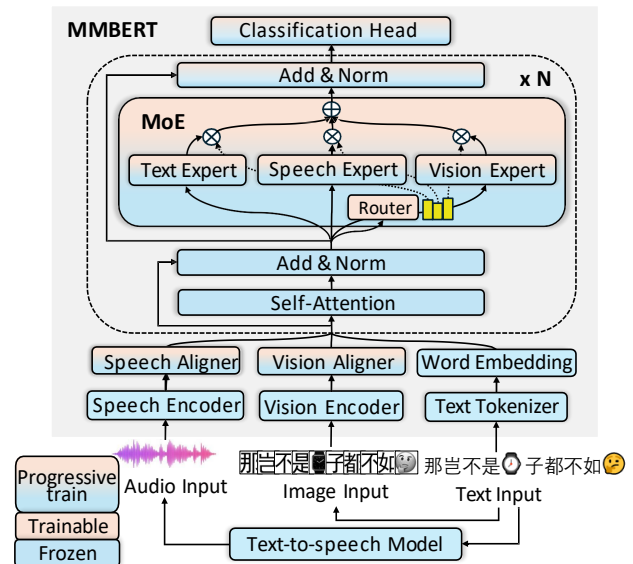
Figure 1: Illustration of MMBERT model structure. Compared to traditional BERT-based model, it leverages the MoE architecture to scale and effectively handle multiple modalities.
