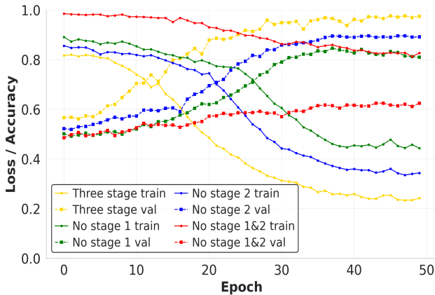
Figure 4: Ablation study evaluating the impact of each stage in the proposed three-stage training strategy
