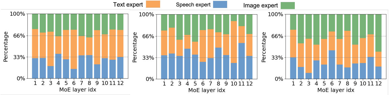
Figure 3: Distribution of expert loading with different input perturbation types, left : non perturbation, middle : homophonic perturbation, right : code-mixing perturbation
