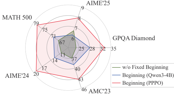
Figure 5: Task performance of Qwen2.5-7B-Instruct when reasoning from prefix tokens extracted from Qwen3-4B with and without PPPO training.
