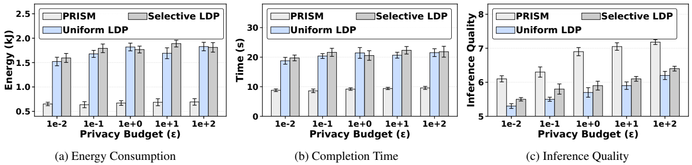
Figure 3: Comparison of privacy-preserving methods across privacy budgets on three dimensions: (a) energy consumption in kilojoules, (b) completion time in seconds, and (c) inference quality evaluated by an LLM as a judge.
