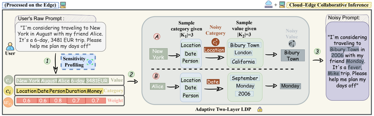
Figure 2: Adaptive Two-Layer LDP for Entity Obfuscation
