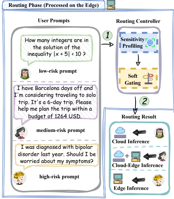
Figure 1: Illustration of the PRISM routing phase. Each user prompt is first analyzed by the edge-side controller, which performs entity-level sensitivity profiling and entropy-regularized soft gating. Based on the inferred privacy risk, the system produces a probability distribution over three execution paths: direct cloud inference, cloud–edge collaboration, and edge-only processing.
