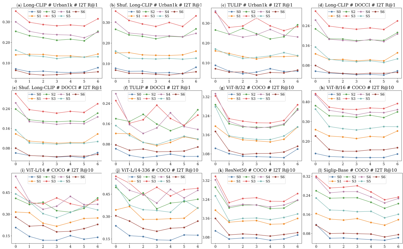
Figure 4: Position bias analysis of image encoders across models and datasets. Each figure title follows the format: model name # dataset # metric. The x-axis shows positions, and colors indicate different segments.
