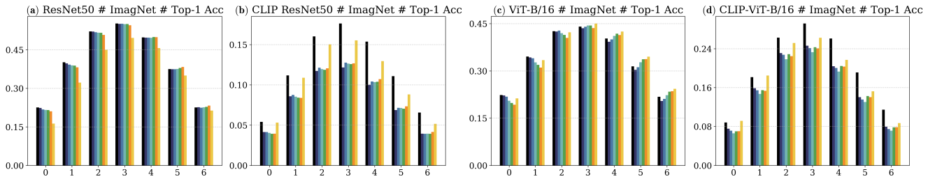
Figure 5: Classification performance on ImageNet for vision-only and CLIP-based models. We report Top-1 accuracy for ResNet-50 and ViT-B/16, both as standalone vision models and as vision backbones within CLIP. Within each bar group, bars correspond to different shift positions along the input.
