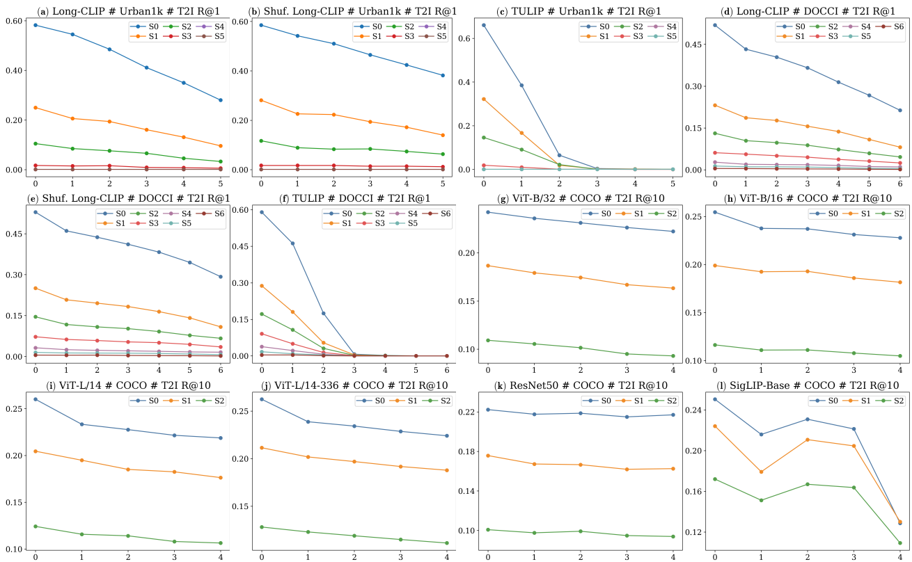
Figure 3: Positional bias analysis of text encoders across multimodal models and datasets. Each figure title follows the format: model name # dataset # metric. The x-axis shows positions, and colors indicate different segments.
