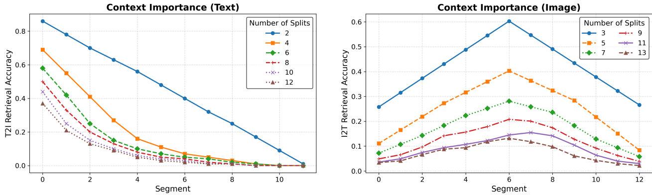
Figure 2: Contextual importance analysis across modalities (image and text). The x-axis shows positions, and colors indicate different number of splits.
