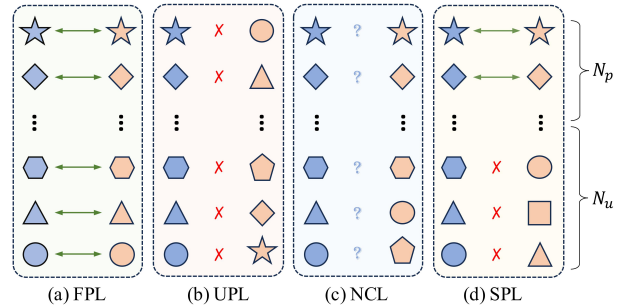
Figure 1: Examples of different cross-modal learning paradigms. Each shape represents an instance, each color denotes a modality ( e.g. , image or text), the green solid line indicates paired correspondence, the red cross indicates unpaired correspondence, and the blue question mark means that the correspondence is unknown/noisy. (a) fully-paired cross-modal learning (FPL), where all pairs are perfectly matched; (b) unpaired cross-modal learning (UPL), where all data are unpaired; (c) noisy correspondence learning (NCL), where alignment information of all data is noisy and unknown; (d) our studied paradigm, i.e. , semi-paired cross-modal learning (SPL), where the number of matched pairs is much smaller than that of unmatched ones, i.e. , N_p \ll N_u .
