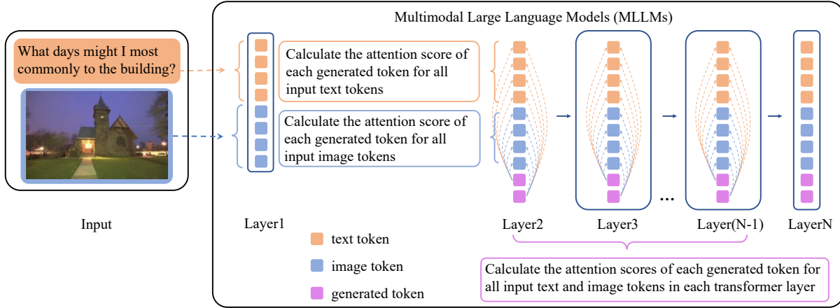
Figure 2: Illustration of the CMAB (Cross-Modality Attention Balance) method. For each generated token, we calculate its average attention score over the input text tokens and image tokens across all transformer layers, and then average these scores across all generated tokens. N represents the total number of layers of the transformer.
