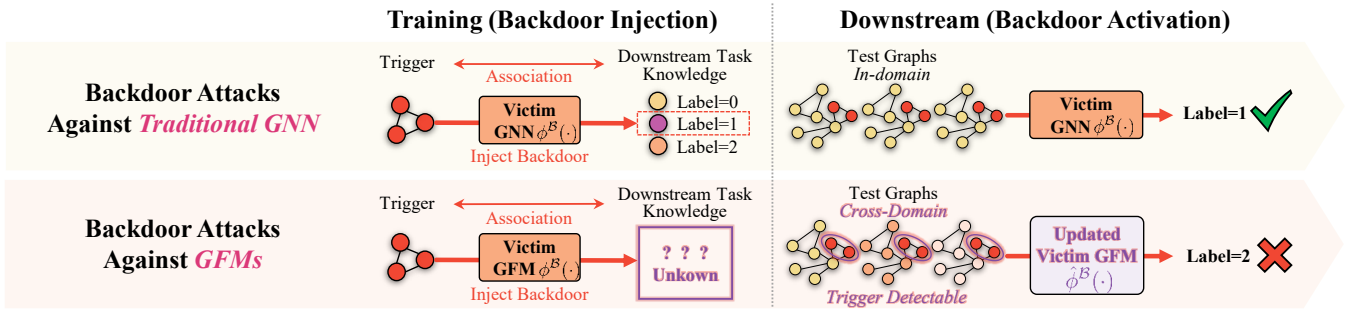
Figure 1: Key differences between backdoor attacks against traditional GNNs and GFM.
