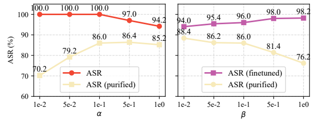
Figure 5: Hyperparameter study on the Photo dataset.
