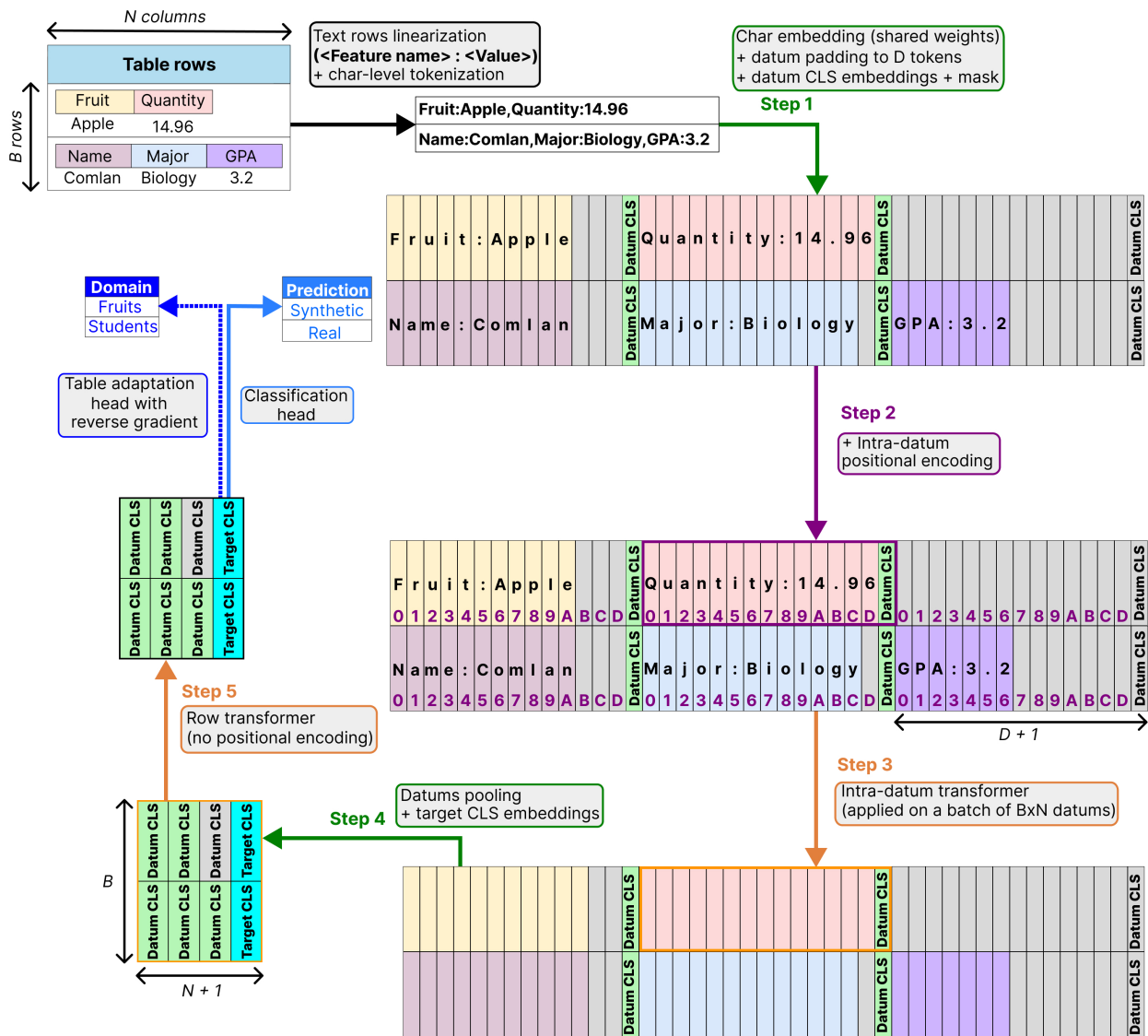
Figure 2: Datum-wise transformer pipeline with table adaptation head.
