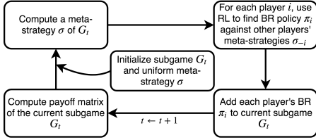
Figure 1: The PSRO framework
