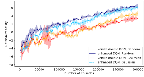
Figure 6: The learning curves of patroller DQNs against parameterized heuristic random walk poachers on 7 \times 7 grids, averaged across four runs.
