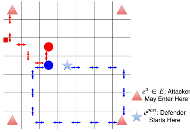
Figure 2: Illustration of GSG-I. The red dot and blue dot represent the attacker and defender respectively. The red arrows and blue arrows represent their corresponding footprints. The red squares on the upper left corner of some cells represent the attack tools placed by the attackers. Each player only observes the opponent’s footprint in their current cell.
