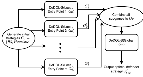
Figure 4: The DeDOL Algorithm
