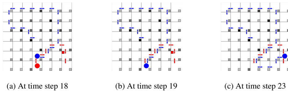
Figure 7: The learned patroller DQN strategy against a parameterized heuristic random walk poacher on a 7 \times 7 random grid world. Here, the darkness of the square in each cell indicates the animal density.
