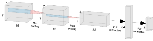
Figure 3: The defender’s neural network architecture for the 7 \times 7 grid.
