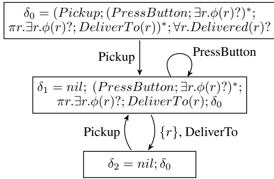
Figure 1: Program graph for the coffee-delivery robot.
