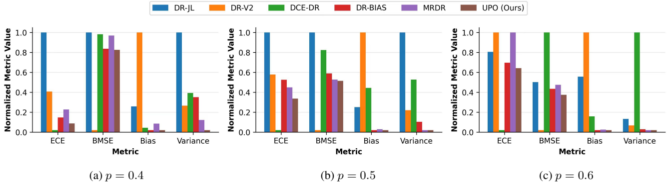
Figure 1: The performance of four metrics and six DR-based debiasing estimators under varying simulated propensity. The propensities are simulated by p^k , where k = 1, 2, 3, 4 corresponds to ratings \{5, 4, 3, 2, 1\} . The methods from left to right are DR-JL (blue), DR-V2 (orange), DCR-DR (green), DR-BIAS (red), MRDR (purple), and UPO (ours, brown).
