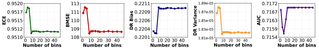
Figure 3: Sensitivity of UPO to the number of bins M on Yahoo! R3 . We report five evaluation criteria, ECE, BMSE, bias, variance, and AUC , as M increases from 1 to 45 on Yahoo! R3 dataset. Performance stabilises once M \geq 10 .
