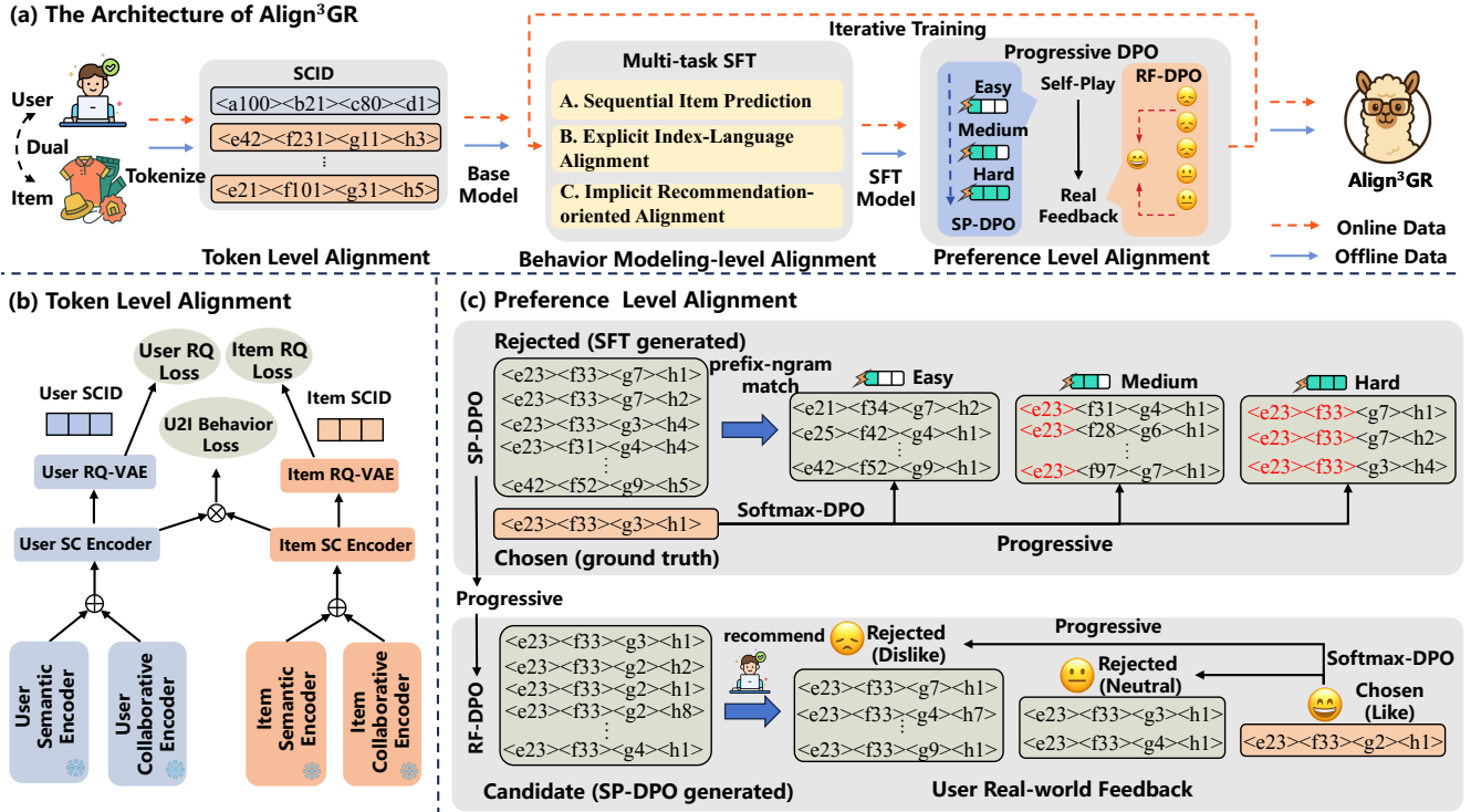
Figure 2: (a) The architecture of Align 3 GR , a unified multi-level alignment framework for generative recommendation, which integrates hierarchical dual SCID, multi-task SFT, and progressive DPO. (b) Token-level alignment is achieved through user-item dual SC encoders and RQ-VAEs. (c) Preference-level alignment is accomplished via progressive SP-DPO and RF-DPO.
