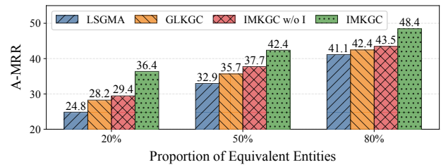
Figure 4: Results (%) with limited equivalent entities, randomly selected at 20%, 50% and 80% on DBP-5L.
