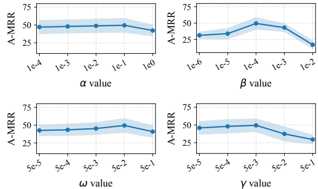
Figure 5: Impact of trade-off factors \alpha, \beta, \omega and \gamma . Averaged MRR (%) is reported with \pm std of 5 KGs in DBP-5L.
