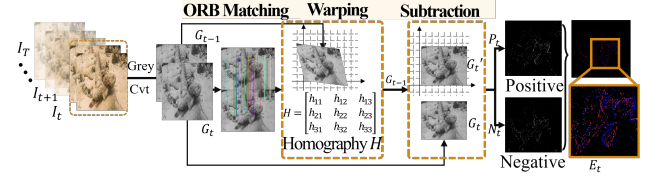
Figure 3: eventstream-inspired Data Extraction Pipeline. The pipeline compensates for global motion and highlights local motion residuals to obtain eventstream-inspired representations from adjacent frames. (zoom in for details)
