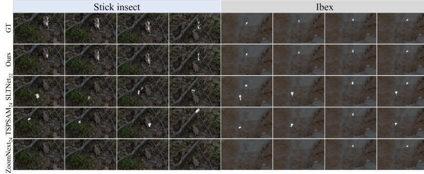
Figure 5: Qualitative results on MoCA-Mask for two challenging scenarios. From top to bottom: Ground Truth (GT), Ours, SLTNet, TSP-SAM, and ZoomNeXt. Each column corresponds to a different frame index. (zoom in for details)
