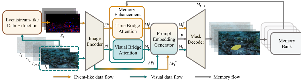
Figure 2: Overview of our framework with two branches: an eventstream-inspired branch for motion modeling and a visual branch for appearance. Both interact with memory through bridge attention and generate adaptive prompts for mask prediction.
