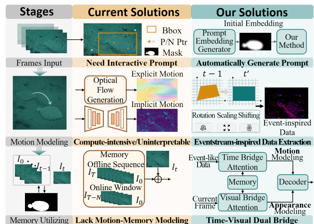
Figure 1: Comparison of existing solutions and our method across three VCOD stages: frame input, motion modeling, and memory utilization. Our approach removes manual prompts, leverages interpretable eventstream motion modeling, and integrates motion cues into long-term memory.
