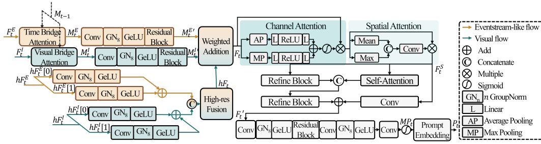
Figure 4: Architecture of the Prompt Embedding Generator (PEG). It fuses event, image, memory, and high-resolution features to generate a feature-level prompt embedding P_t for segmentation. (zoom in for details)
