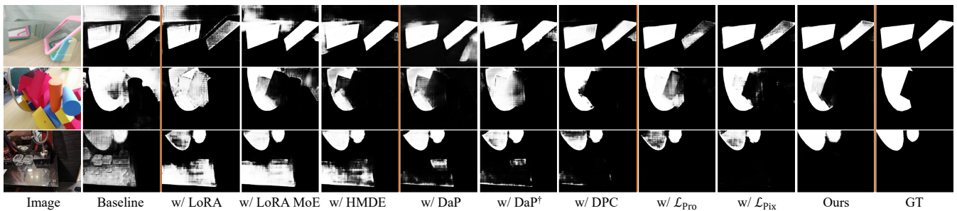
Figure 3: Qualitative ablation of proposed components. From top to bottom, the scenes include cross-imaging, complex correspondence and occlusion, and smooth tabletop reflection interference. Partial variants correspond to Table 4.
