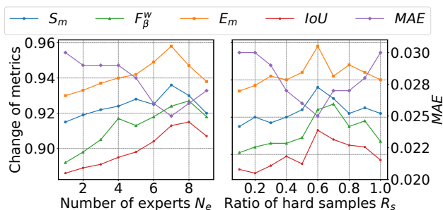
Figure 4: Ablation of hyperparameter settings on the MSD.
