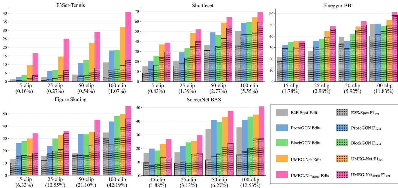
Figure 3: F1_{\text{evt}} and Edit scores under few-shot ( k -clip) training. Percentages indicate the fraction of the full training set.
