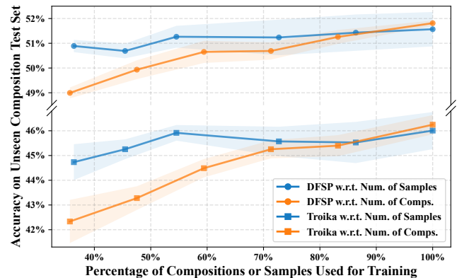
Figure 1: Accuracy of CZSL models on the unseen composition test set trained with data containing varying number of compositions or samples. Increasing training compositions boosts compositional generalization significantly more than increasing training samples.
