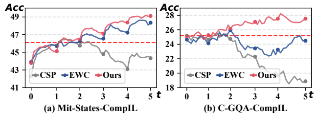
Figure 5: Compositional generalization capability of CSP, equipped with state-of-the-art methods, after training on different tasks in the compositional incremental learning process. The red line indicates CLIP’s zero-shot performance.
