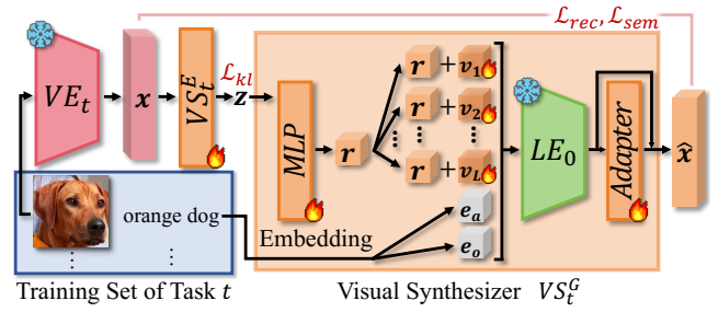
Figure 4: The architecture and training of the visual synthesizer. The visual synthesizer comprises an encoder VS_t^E and a generator VS_t^G . It is trained to synthesize visual representations conditioned on the given composition name.
