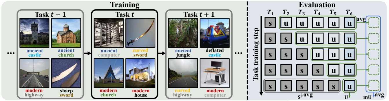
Figure 2: Illustration of our CompIL setting, taking the proposed MIT-States-CompIL benchmark as an example. The left side illustrates training samples from the tasks, where samples from different tasks vary significantly in semantics. For instance, the attribute “ancient” describes buildings in task t - 1 , outdated technology in task t , and natural landscapes in task t + 1 ; the object “castle” varies likewise. The right side depicts the evaluation process, with rows representing training steps and each column indicating performance on the corresponding task.
