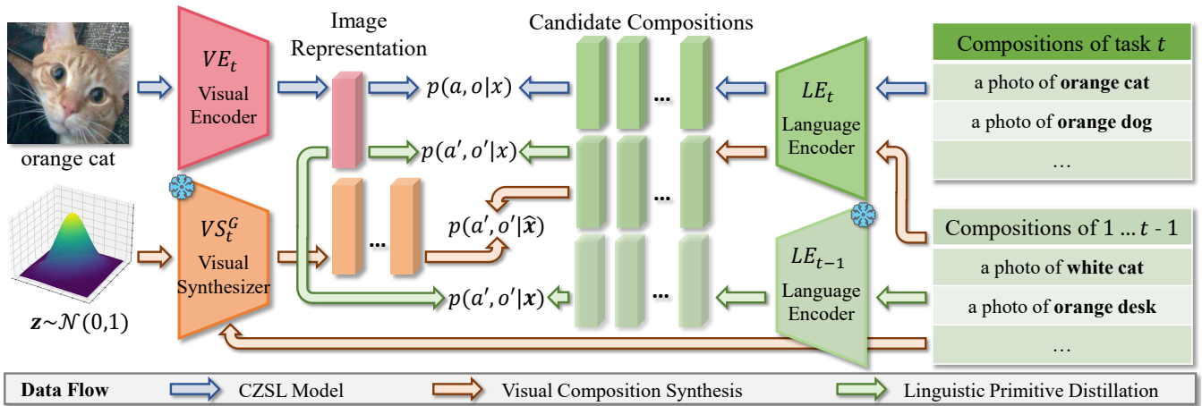
Figure 3: Overview of the pseudo-replay framework in the context of compositional zero-shot learning. The CZSL model contains a visual encoder VE_t and a language encoder LE_t . For simplicity, we omit possible connections between two components.
