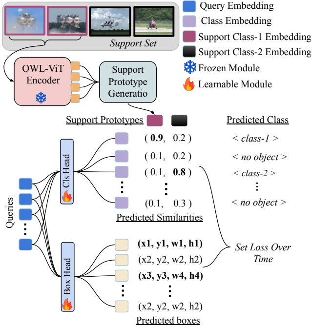
Figure 3: Few-shot Classification and Detection Heads. Our architecture processes object queries through parallel projection heads for classification and localization. Classification embeddings are compared against support embeddings via cosine similarity, while the detection head predicts bounding box coordinates. The temporal consistency is maintained by propagating matched object queries.
