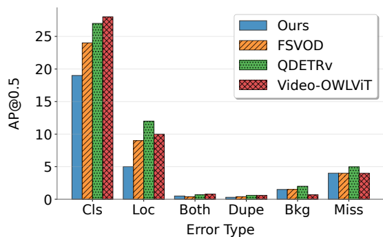
Figure 6: Error type analysis on FSVOD val set.
